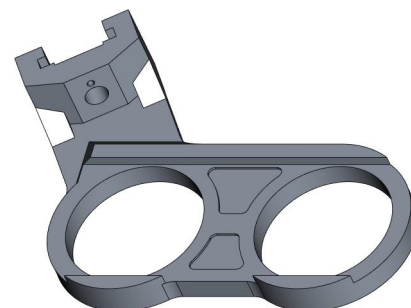
Main body KV-401-017-001
