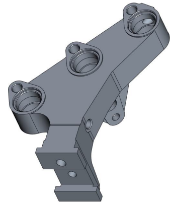
Main body KPG-401-003-001
