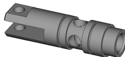
Head stem KPG-401-003-003-001
