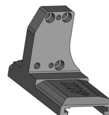
Left bracket DGK-401-010-003
