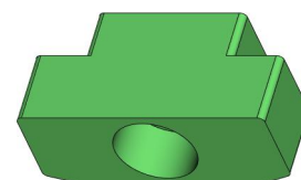
Bushing DF-401-011-004
