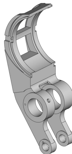
Lower lever DF-401-041-001
