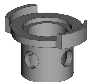
Sleeve PPL-401-034-002
