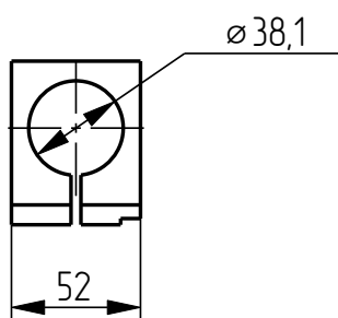
13. Holder KDG-401-012-003
