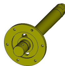
7. Pinion shaft RD-401-005-040
