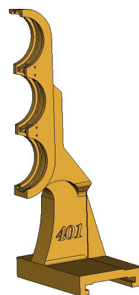
5. Neckring holder RH DGK-401-015-001
