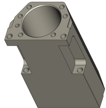
Cylinder MPL-401-010-003-001
