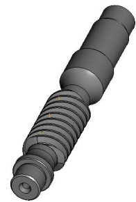
3. Worm shaft D-72135-401-03M2Z3
