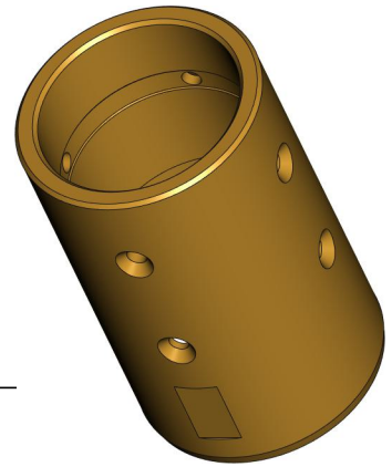
Bushing DF-401-001-005
