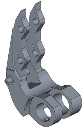
Upper lever DF-401-022-002
