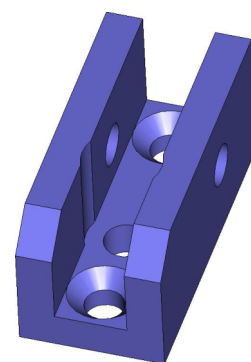
4. Holder KDG-401-007-004
