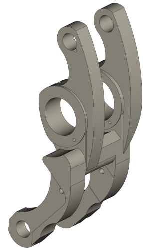
Lower lever DF-401-006-002
